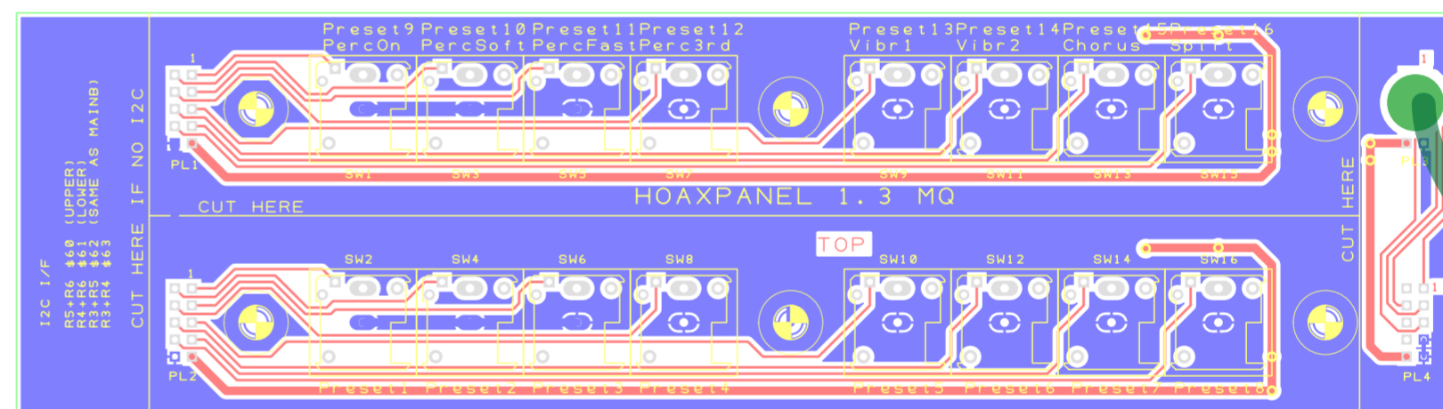
Preset Panel Upper
