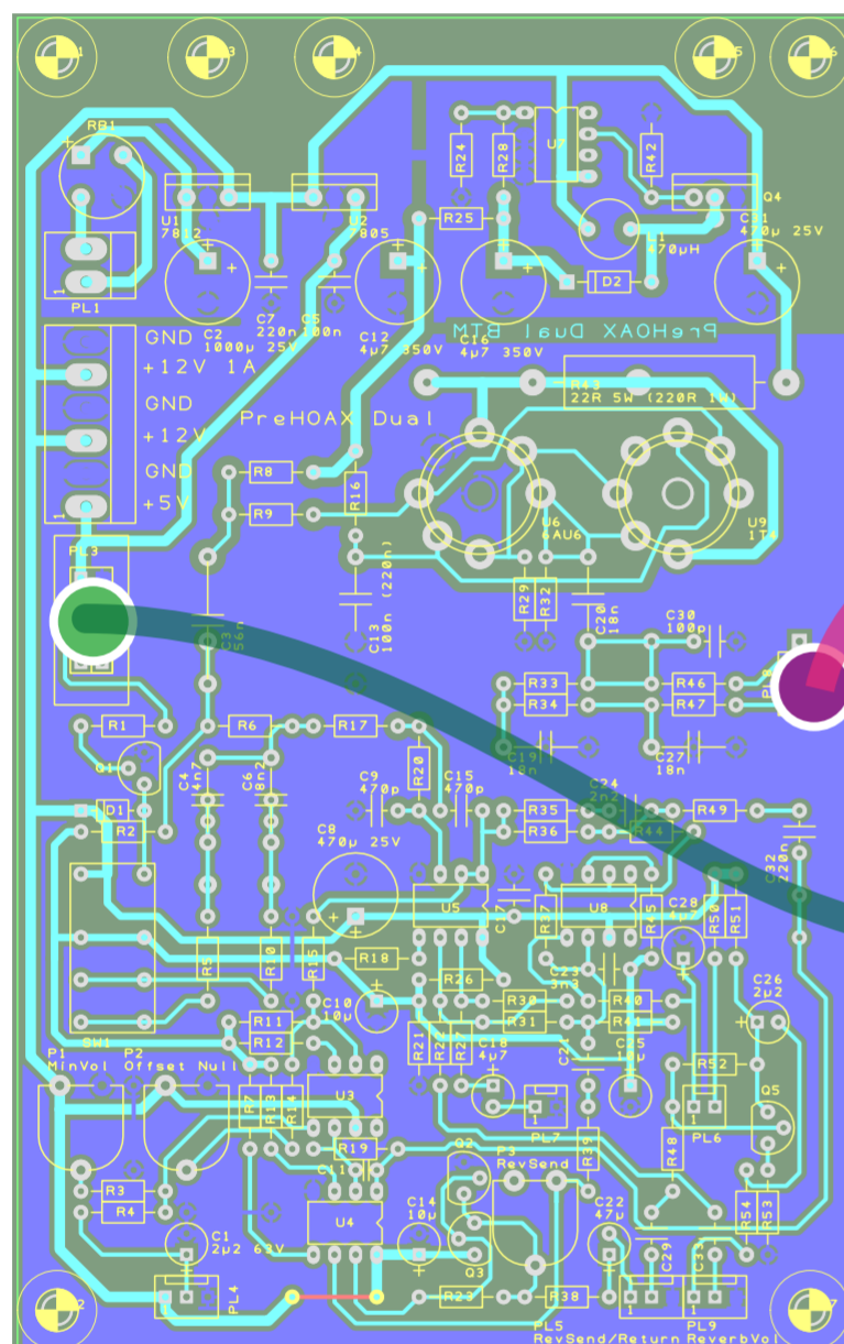
PreHOAX Tube Preamp
